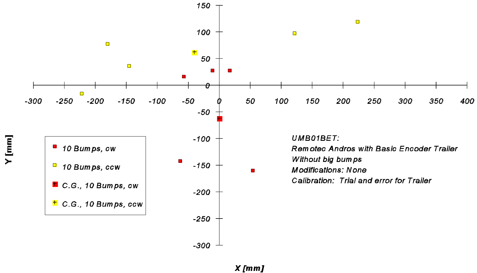
Figure C-5: Return Position Errors for the Remotec Andros with Basic Encoder Trailer. UMBmark test with 4×4 m bi-directional square path. Smooth concrete floor, no bumps. We hypothesize that the large spread of return position errors is a measuring error caused by wear in the slip-ring mounted on the joint between Andros platform and encoder trailer.
