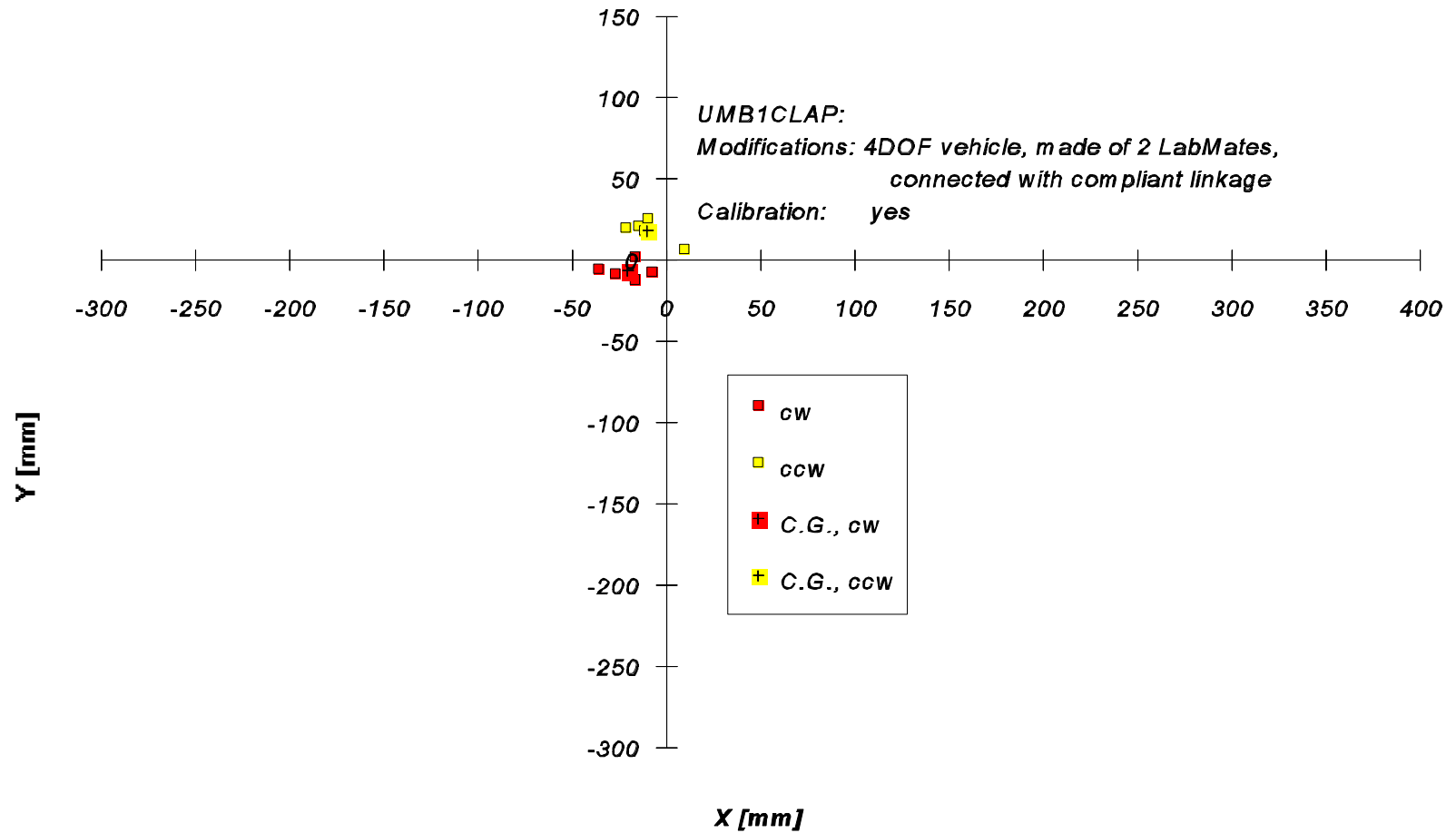
Figure C-3: Return Position Errors for the University of Michigan's CLAPPER. UMBmark test with 4×4 m bi-directional square path. Smooth concrete floor, no bumps.
