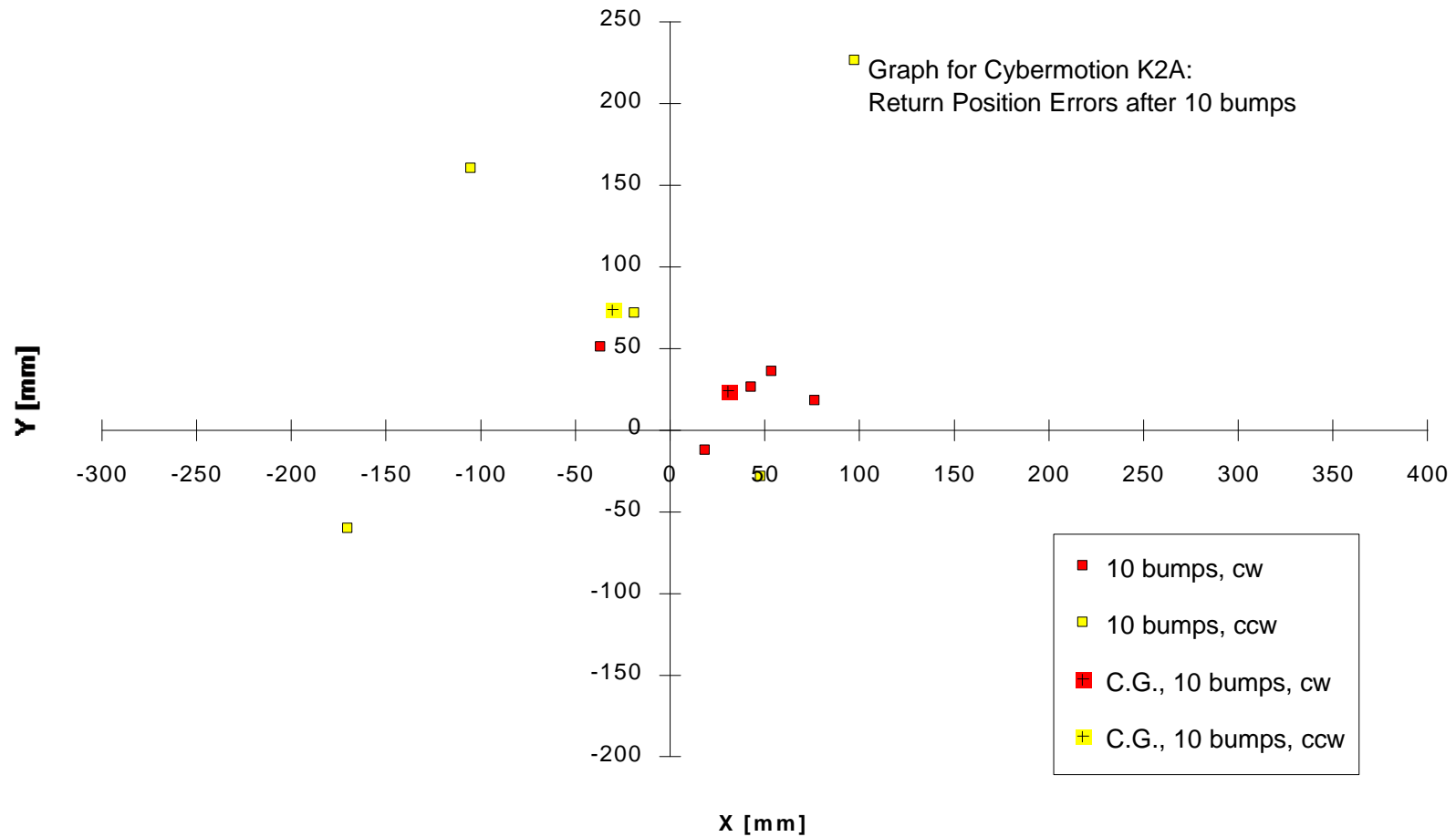
Figure D-2: Return Position Errors for the Cybermotion K2A. Extended UMBmark test with 4×4 m bi-directional square path. 10 bumps, each 10 mm high, were introduced during the first leg. It is difficult to explain the exceedingly wide spread of the return position errors in ccw direction.
