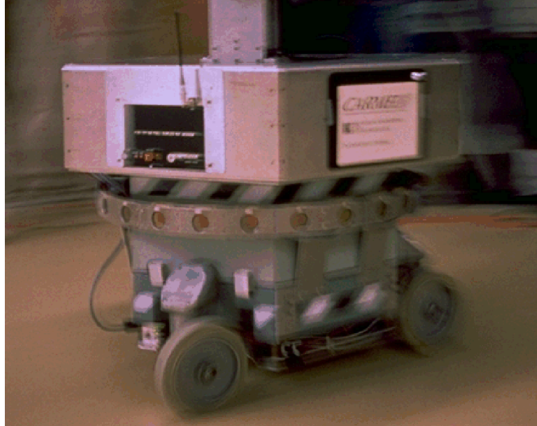
Figure 4.2: CARMEL, the University of Michigan's oldest mobile robot has been in service since 1987. CARMEL is a Cybermotion K2A platform with many custom additions. In 1992 CARMEL was voted one of the 100 "Best of What's New" products in Popular Science .
