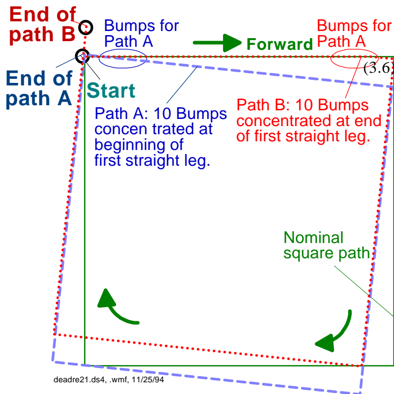
Figure 3.5: The return position of the extended UMBmark test is sensitive to the exact location where the 10 bumps were placed. The return orientation is not.
