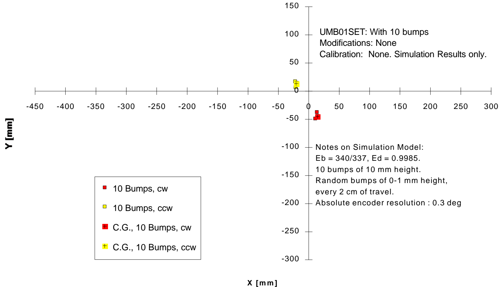
Figure D-6: Return Position Errors for a simulation run with the Smart Encoder Trailer (SET). The Extended UMBmark test with a 4×4 m bi-directional square path was applied, and, in addition, 10 bumps, each 10 mm high, were introduced during the first leg of the square path. The SET uses the same principle of error correction as the CLAPPER. The simulation program is directly derived from a similar simulation for the CLAPPER. Results from the CLAPPER simulation were consistently similar to the actual CLAPPER, increasing our trust in the accuracy of the SET simulation.
