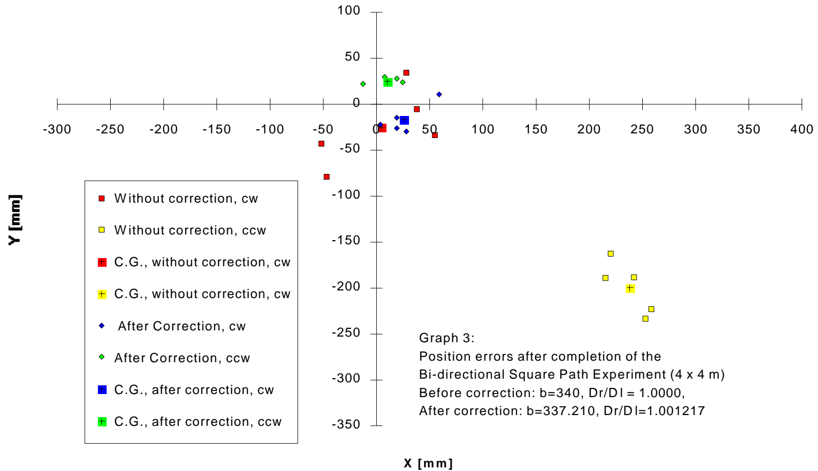
Figure E-3: Experiment E-3 shows yet another set of runs before and after calibration. Here the improvement is 10-fold (the least successful run in this series of eight experiments).
