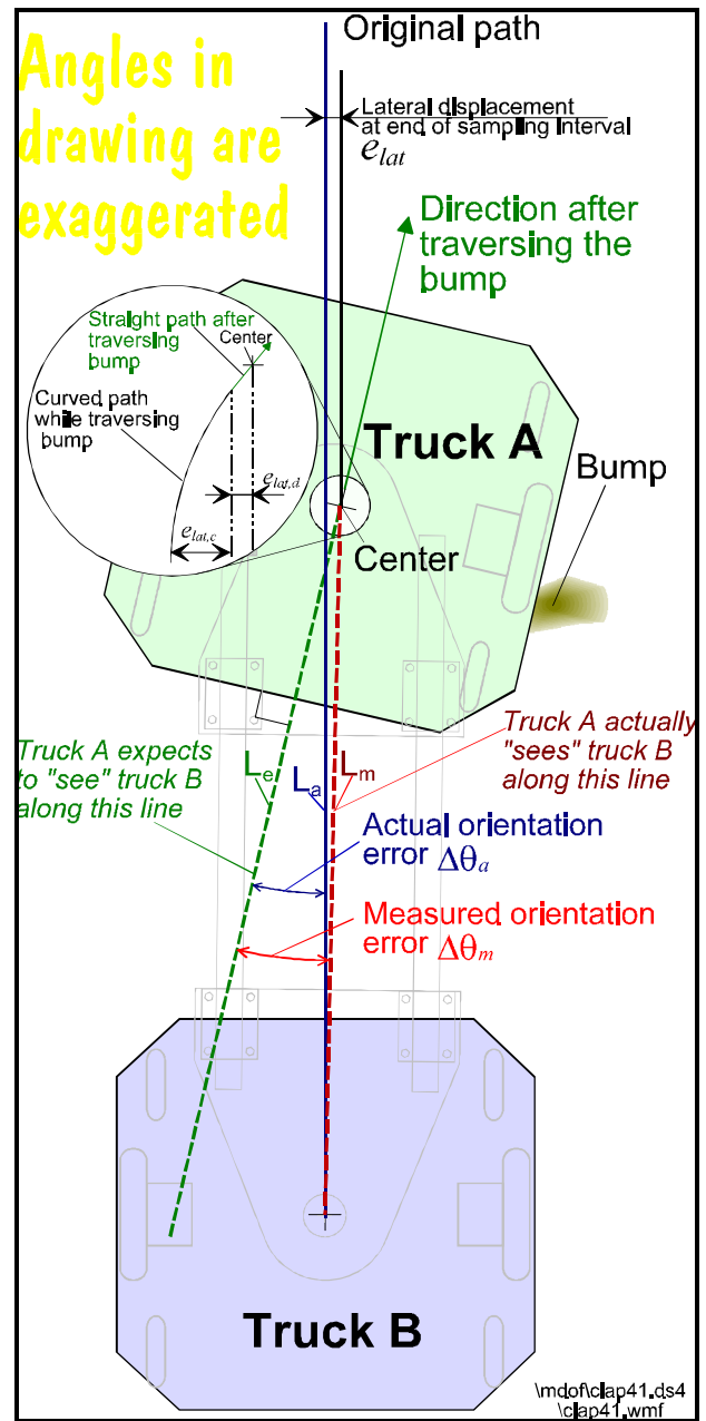
Figure 4: After traversing a bump, the resulting change of orientation of truck A can be measured relative to truck B.
