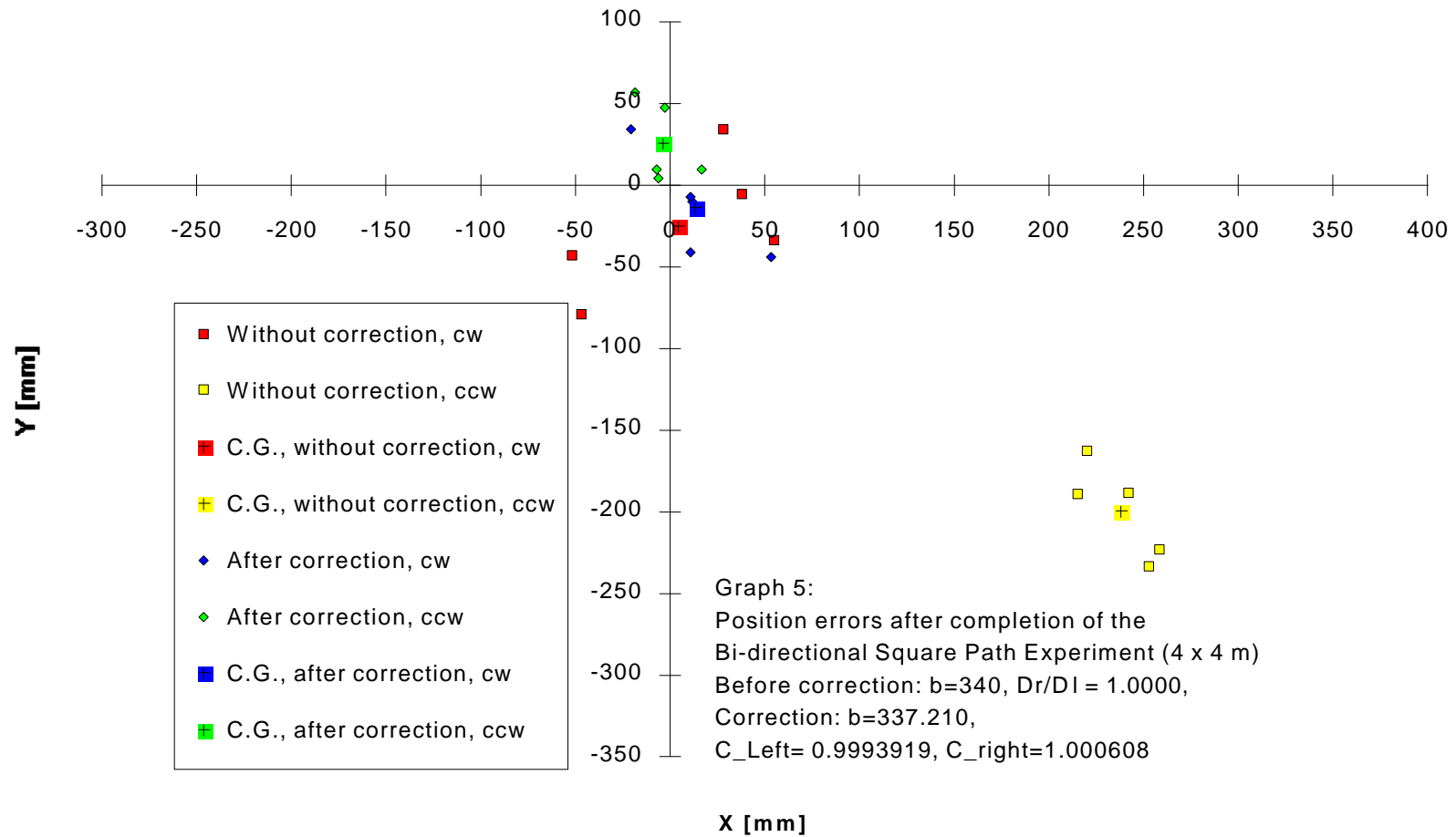
Figure E-5: Once more, the same set of correction factors as in E-3 and E-4 was used. The improvement this time is 12-fold. Experiments E-3, E-4, and E-5 reinforce our observation that the UMBmark calibration procedure provides consistently one order of magnitude improvement in dead-reckoning accuracy (with respect to systematic errors).
