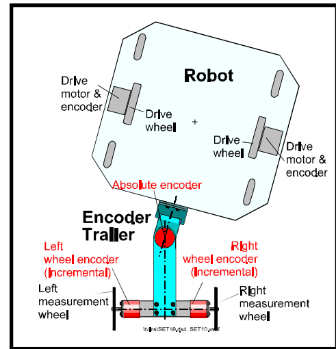
Figure 4.6: Concept drawing of the University of Michigan's Smart Encoder Trailer (SET).
