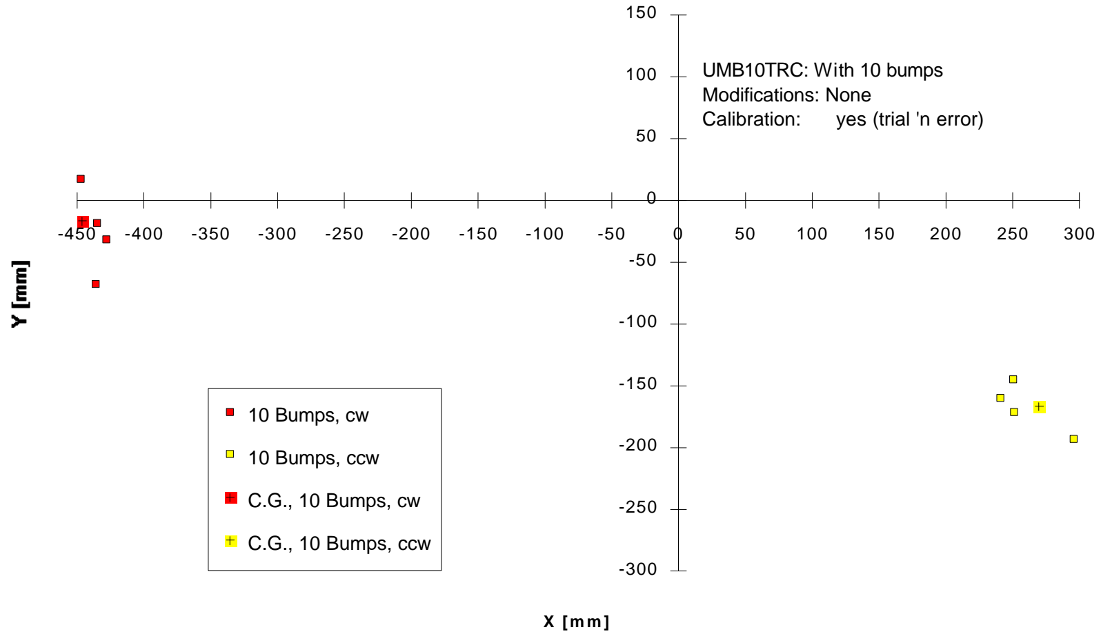
Figure D-1: Return Position Errors for the TRC Labmate Extended UMBmark test with 4×4 m bi-directional square path. 10 bumps, each 10 mm high, were introduced during the first leg.
