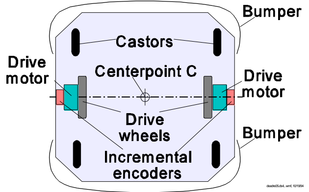
Figure 2.1: A typical differential-drive mobile robot (bottom view).
