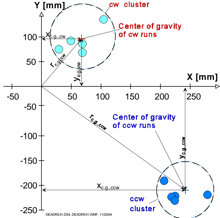
Figure 3.4: Typical results from running UMBmark (a square path run in both cw and ccw directions) with an uncalibrated vehicle.
