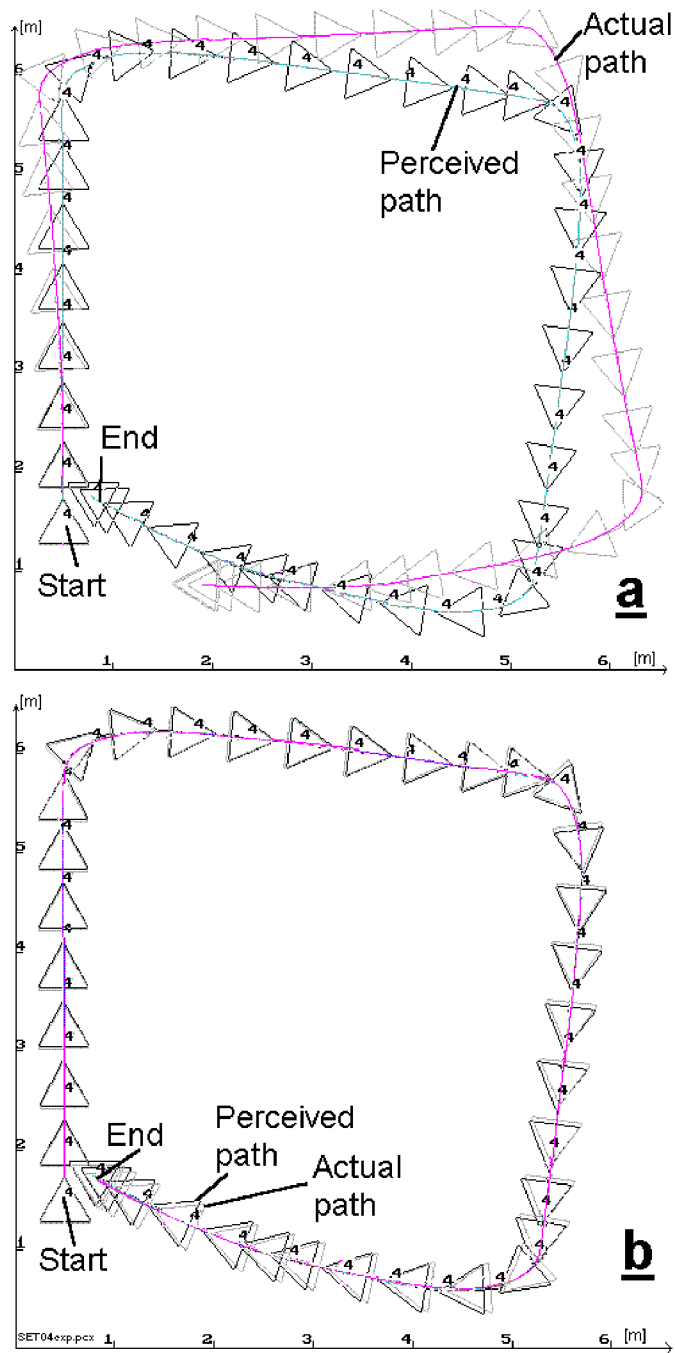
Figure 4.9: The screen shot here was taken after an earlier experiment in which the simulated robot/SET traversed bumps during all 4 legs of the square path. The double images show the difference between "actual" and "perceived" positions of the robot, due to dead-reckoning errors. (a) IPEC disabled , and (b) IPEC enabled .
