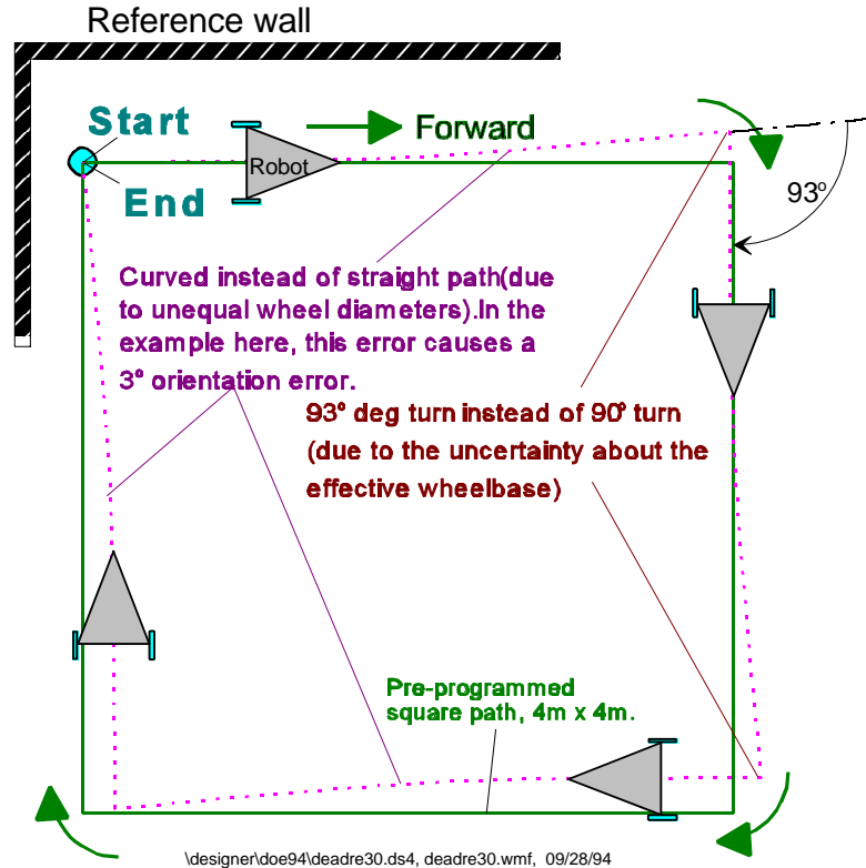
Figure 3.2: The effect of the two dominant systematic dead-reckoning errors E_b and E_d . Note how both errors may cancel each other out when the test is performed in only one direction.
