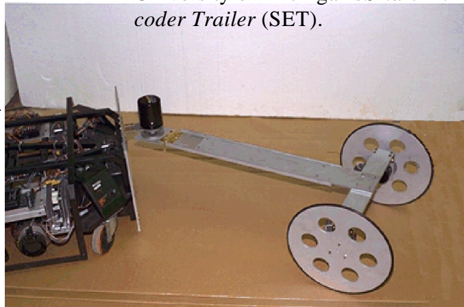
Figure 4.7: Prototype of the University of Michigan's Smart Encoder Trailer (SET). In the photo here, the SET is attached to a TRC LabMate, but the SET's encoders are not interfaced yet. U of M plans to implement the IPEC method in early 1995. Then, if successful, U of M will develop algorithms designed to allow fully transparent backward travel with a trailer.
