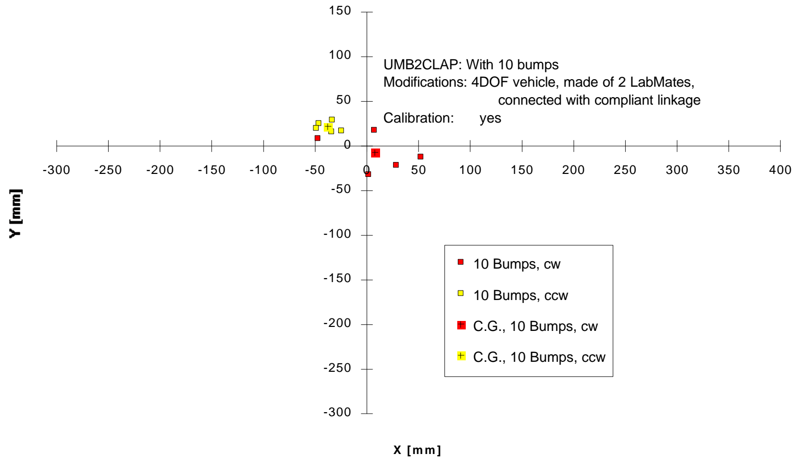
Figure D-3: Return Position Errors for the University of Michigan's CLAPPER Extended UMBmark test with 4×4 m bi-directional square path. 10 bumps, each 10 mm high, were introduced during the first leg. The CLAPPER is especially designed to detect and correct non-systematic dead-reckoning errors. The result: a vehicle that is almost completely resilient to errors due to bumps, cracks, or other irregularities of the floor.
