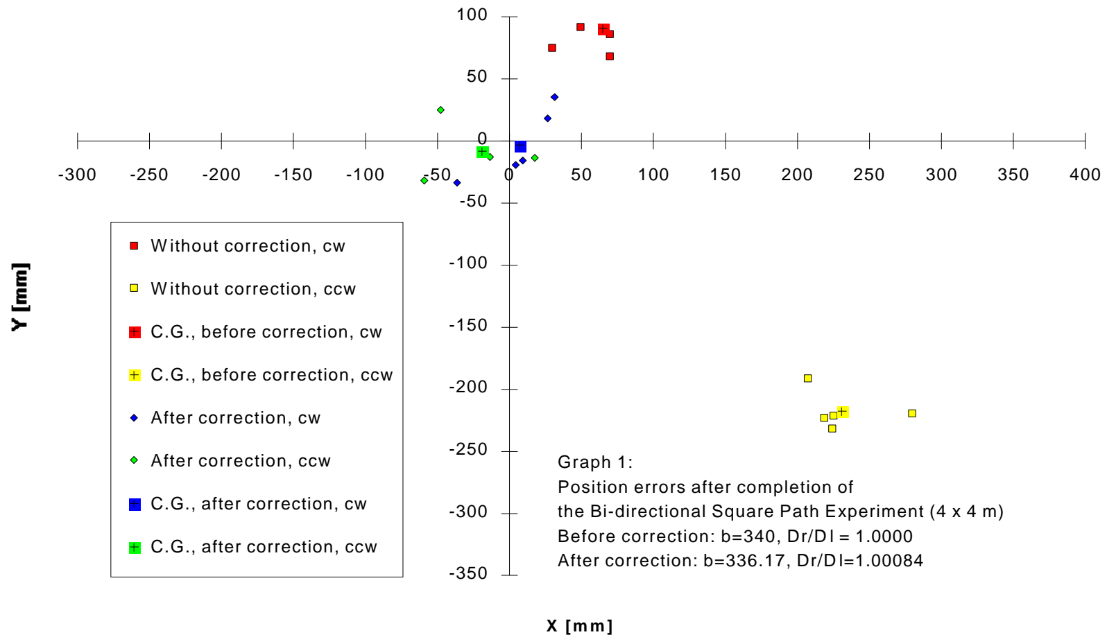
Figure E-1: Experiment E-1 shows how the return position error of the LabMate is reduced dramatically after compensation with the analytical compensation factors derived in Section 6. Here the improvement is 15-fold (Improvement is measured as the ratio between the furthest center of gravity (C.G.) of the uncalibrated runs and the furthest C.G. of the runs after calibration).
