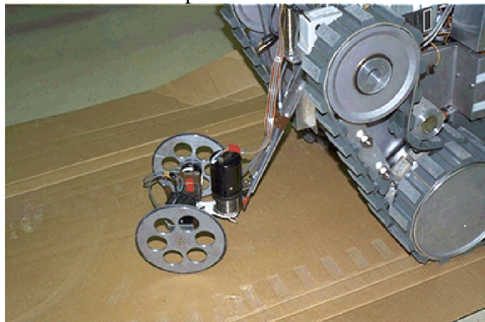
Figure 4.5: This encoder trailer was recently developed at the University of Michigan for use with tracked robots. The trailer is here shown temporarily attached to a TRC LabMate, prior to its permanent installation on the Remotec Andros.
