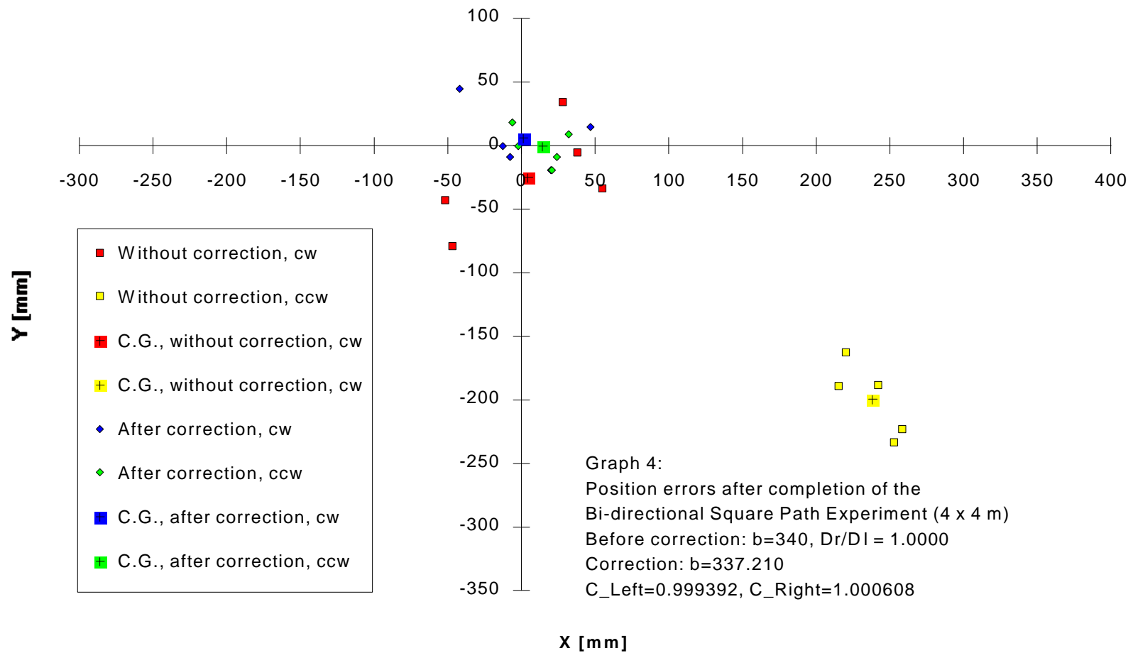
Figure E-4: Same set of correction factors used as experiment 3, but new set of "after-calibration runs." Here the improvement is 21-fold (see text in Section 6.3 for explanation of this seemingly different result, as compared to experiment E-3)
