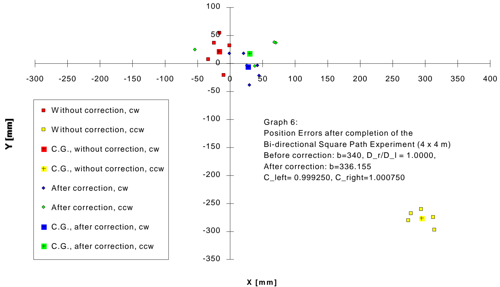
Figure E-6: To test the repeatability of the UMBmark calibration procedure, we ran the procedure again, from the beginning: we ran UMBmark without any correction, derived the correction factors from the results of the UMBmark run, and ran UMBmark again with the computed correction factors. Here the improvement in accuracy was 11-fold.
