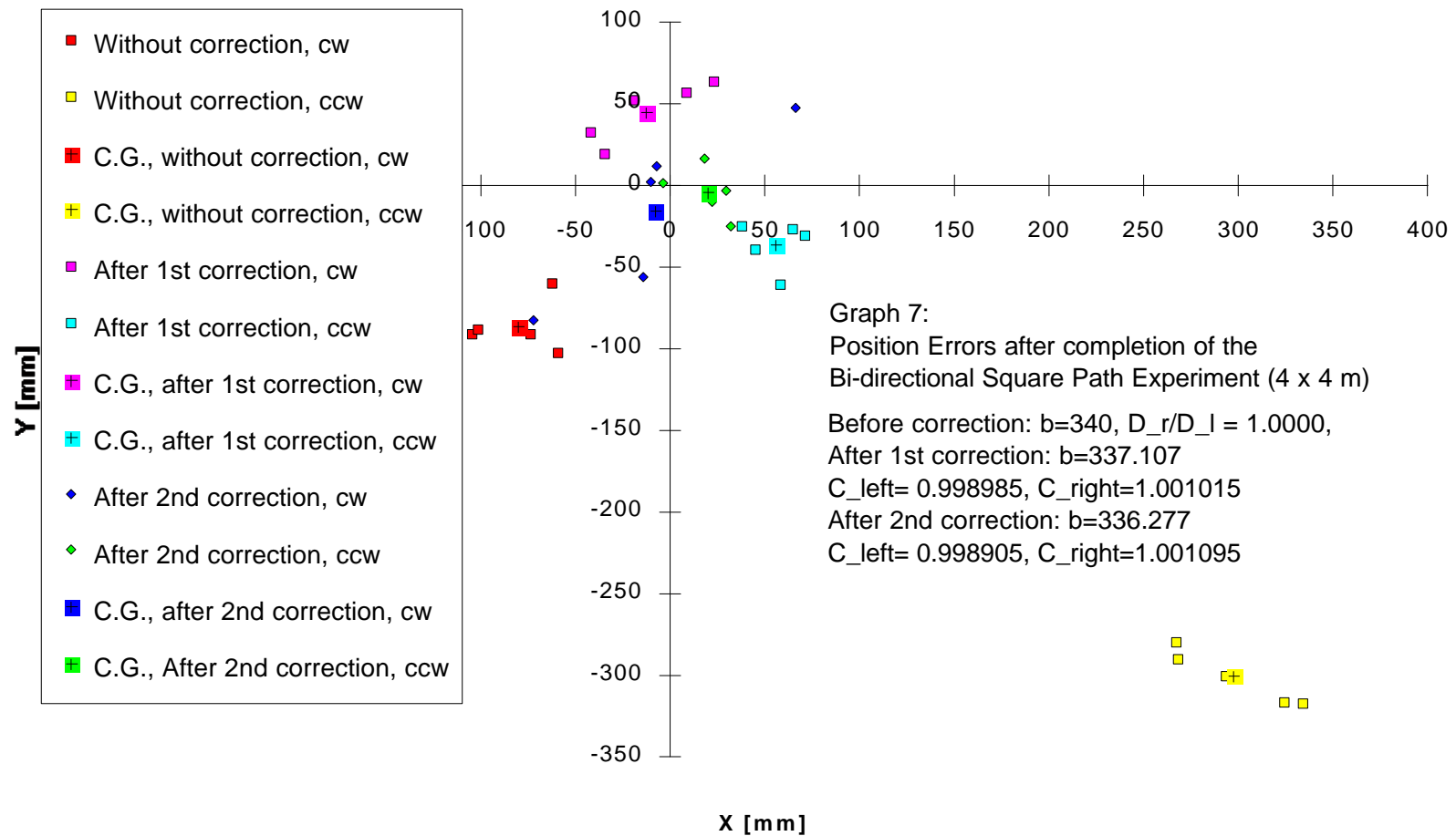
Figure E-7: In this experiment the diameter of the right wheel was slightly increased by winding three loops of masking tape around the wheel perimeter. This results effectively in a "different" vehicle. In this experiment, the initial improvement was only 6-fold. However, applying a simple test (explained in Section 6.3) it is immediately clear that further improvement can be achieved. Applying the UMBmark calibration procedure for a second time, the overall improvement becomes 21-fold.
