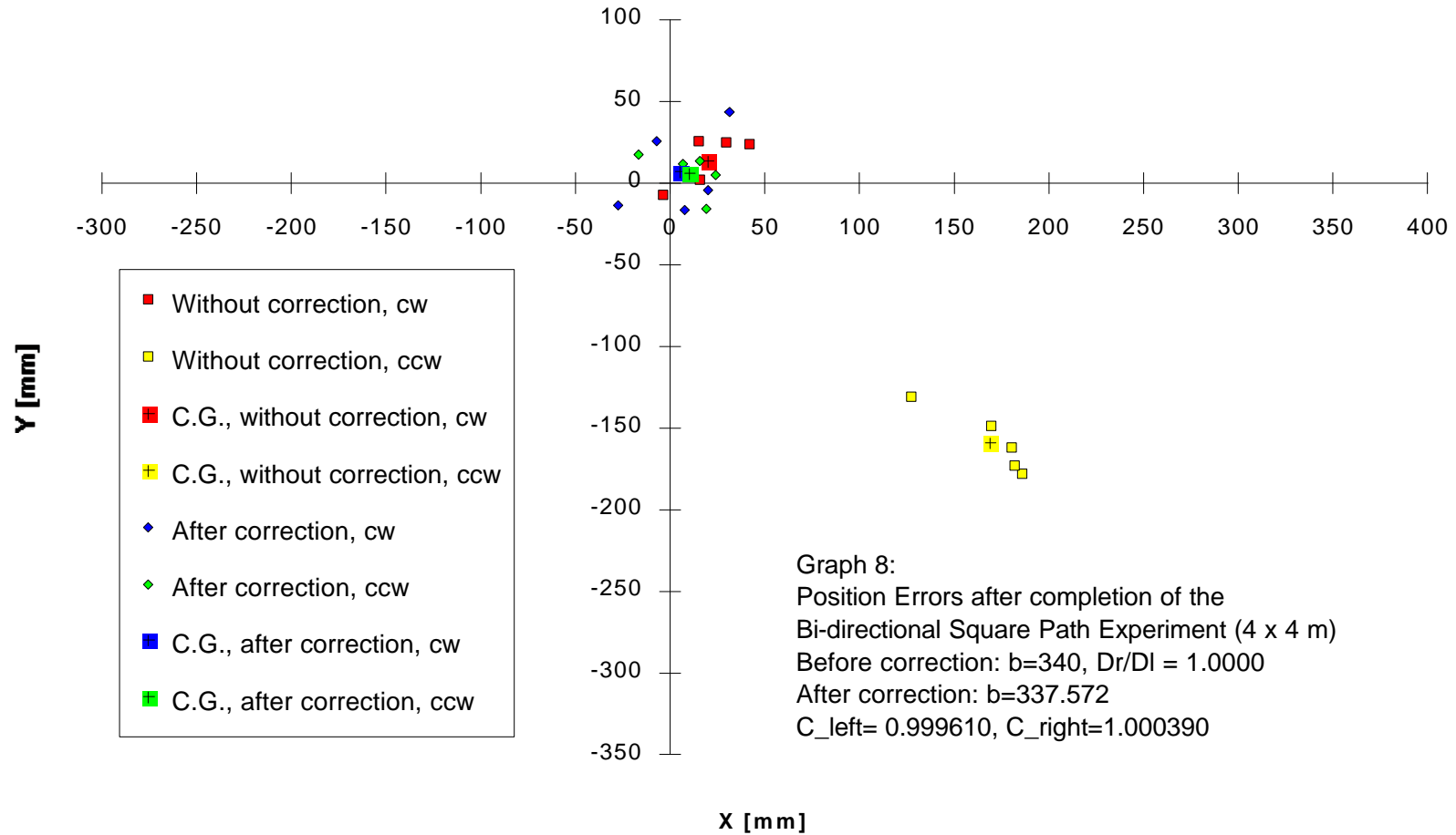
Figure E-8: In this experiment the diameter of the left wheel was slightly increased by winding five loops of masking tape around the left wheel perimeter. The improvement after applying the UMBmark calibration procedure was 19-fold.
