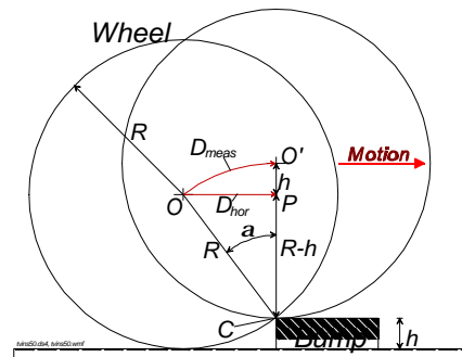
Figure 3: Simplified geometry of wheel traversing a bump.
