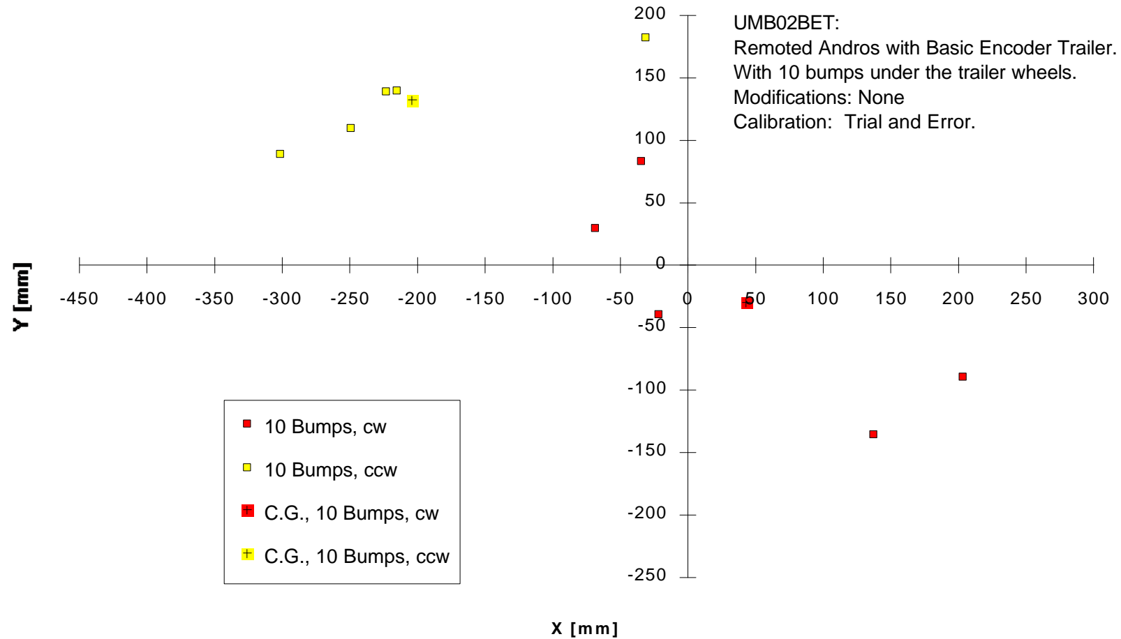
Figure D-5: Return Position Errors for the Remotec Andros with Basic encoder Trailer attached. This test comprised the nominal 4×4 m bi-directional square path. 10 bumps, each 8-9 mm high, were introduced under the trailer's wheels during the first leg of the run.
