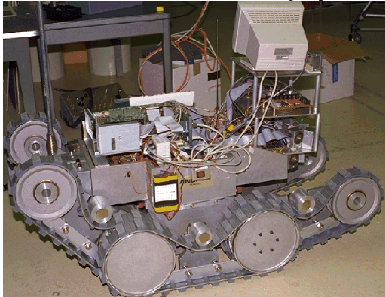
Figure 4.4: The University of Michigan's Remotec Andros is custom equipped with incremental optical encoders on both drive motors and on the auxiliary track motors. The original onboard computer and motor controllers were replaced by a 486-66 MHZ PC-compatible single board computer and our own HCTL 1100-based motor controllers.
