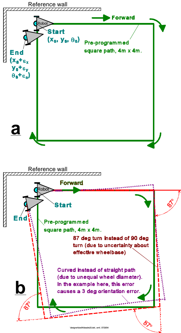
Figure 3.1: The unidirectional square path experiment.
