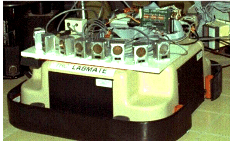
Figure 4.1: One of the four TRC LabMates at the University of Michigan. The system shown here is equipped with 8 ultrasonic sensors that were not used in the UMBmark experiment.
