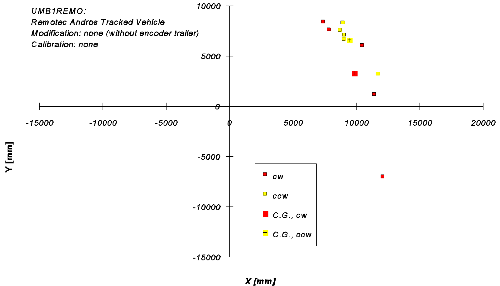
Figure C-4: Return Position Errors for the Remotec Andros. UMBmark test with 4×4 m bi-directional square path. Smooth concrete floor, no bumps. Note that the scale of this plot is 50 times coarser than that of all other plots. The typical return position error of the tracked Andros vehicle was on the order of 8-10 meters! The average orientation error was 130°! Clearly, dead-reckoning with a tracked vehicle is out of the question.
