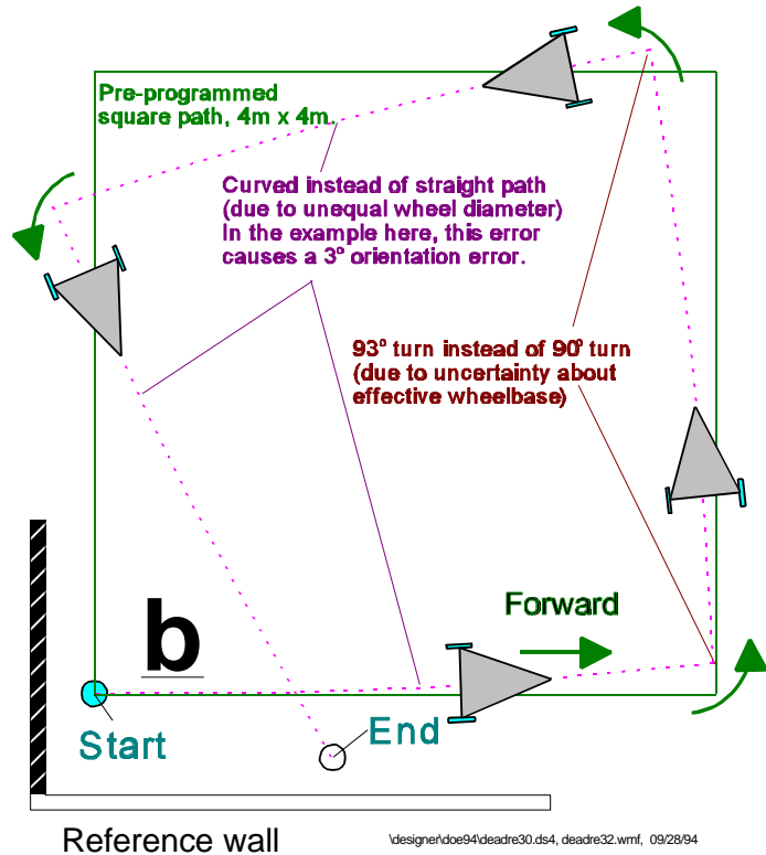
Figure 3.3: The effect of the two dominant systematic dead-reckoning errors E_b and E_d : When the square path is performed in the opposite direction one may find that the errors add up.
