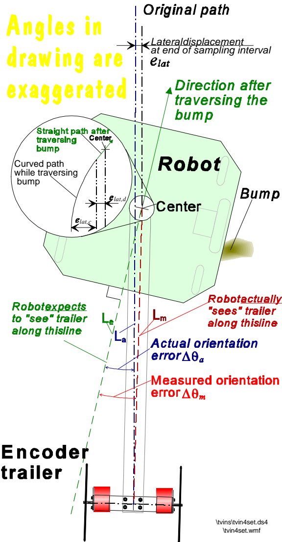
Figure 4.8: After traversing a bump, the resulting change of orientation of the robot can be measured relative to the trailer (for simplicity shown with the absolute encoder at the robot's center).
