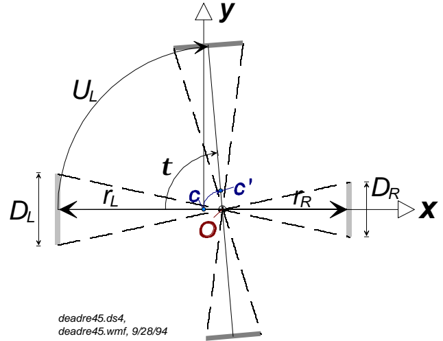
Figure A1: When turning through a nominal 90^\circ turn, it is not the "unequal wheel diameter" error, but rather the "average actual wheel diameter" error, that affect the amount of turning.
