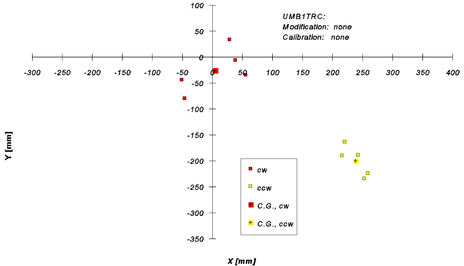
Figure C-1: Return Position Errors for the TRC LabMate. UMBmark test with 4×4 m bi-directional square path. Smooth concrete floor, no bumps.
