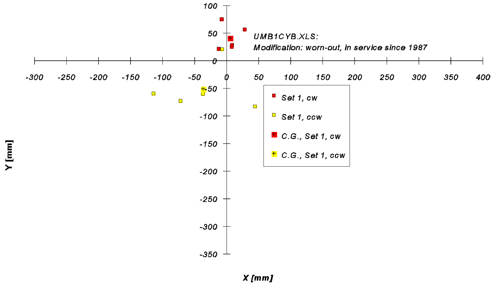
Figure C-2: Return Position Errors for the Cybermotion K2A. UMBmark test with 4×4 m bi-directional square path. Smooth concrete floor, no bumps.
