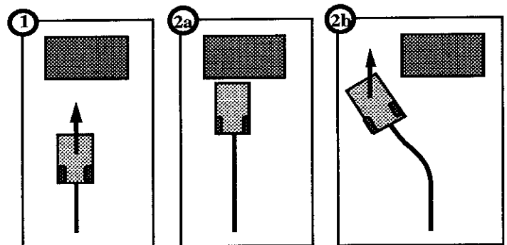
Figure 1: Mode Selection. The NavChair must be able to perform mode selection in the absence of environmental cues. Frame (1) shows the NavChair approaching a desk. One of two outcomes is possible: either (2a) the NavChair 'docks,' allowing the user to access the desk, or (2b) the NavChair performs an avoidance maneuver and continues to move forward. These two behaviors correspond to two different modes of operation, close approach and obstacle avoidance, that cannot be performed simultaneously.
