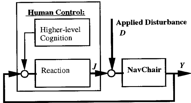
Figure 2: Human Reactive Control Loop. The human reactive control loop is where deviations from the target path are perceived and corrected: the actual motion of the chair, Y , is compared to the target path, T , to produce a joystick command, J . Observations of responses to an applied disturbance, D , are used to model the behavior of this feedback loop.
